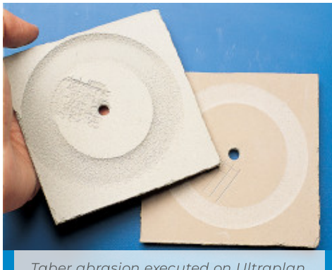
Taber abrasion executed on Ultraplan (right specimen) and on conventional levelling (left specimen) after 200 cycles
