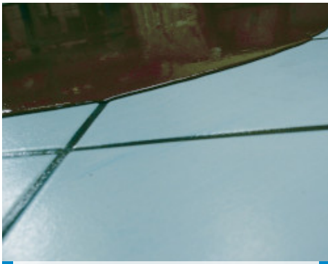
Detail of the application of Ultraplan on an existing ceramic tile floor after the application of Eco Prim T Plus
